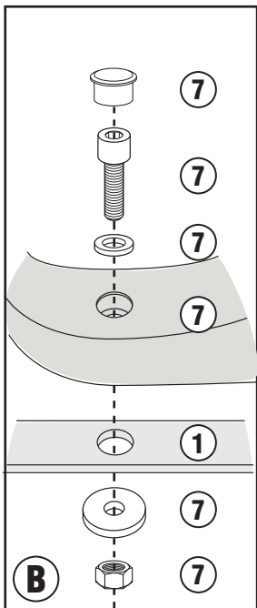
M5/M6M/M7/M5M PLATES
